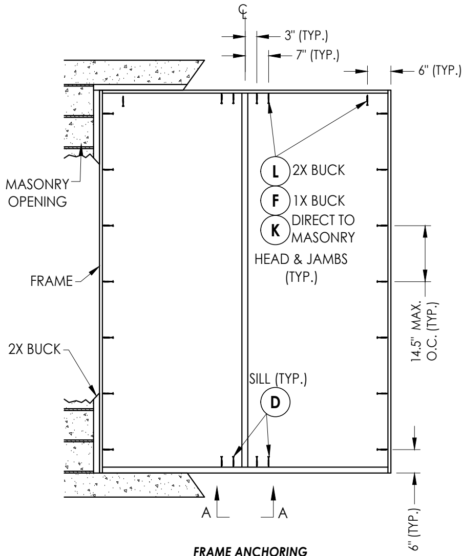
FRAME ANCHORING
