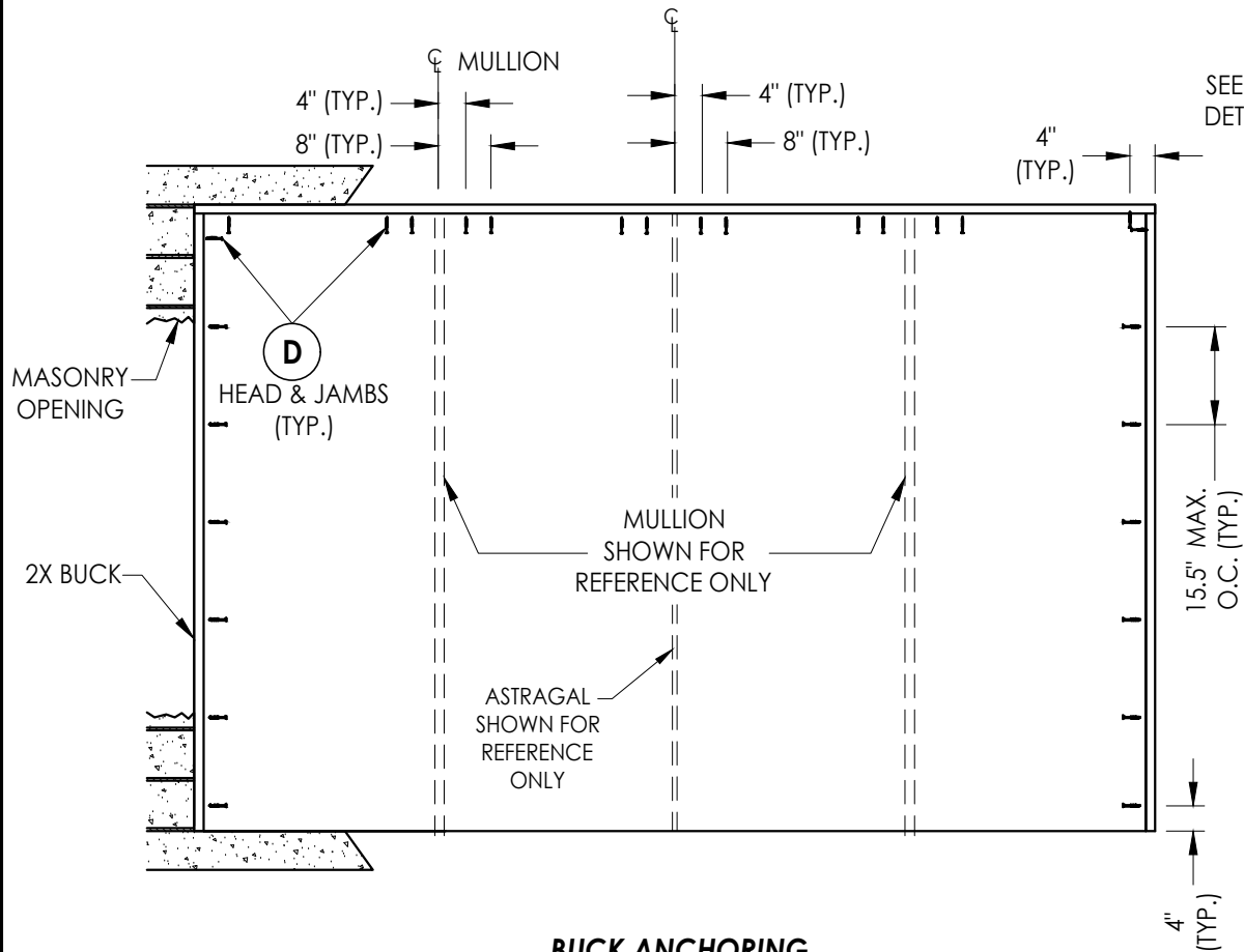
BUCK ANCHORING
