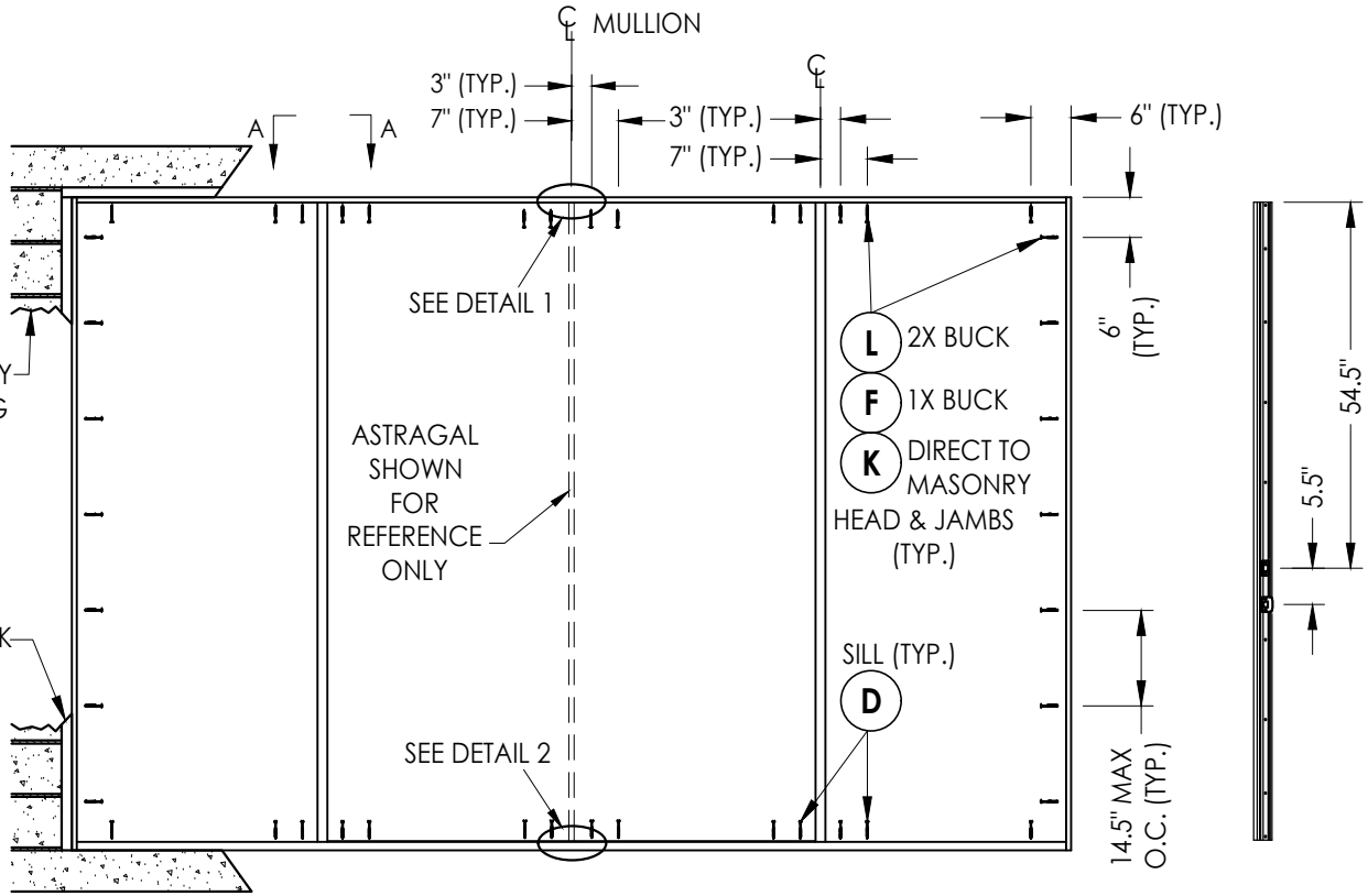
FRAME ANCHORING Masonry construction
