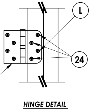
HINGE DETAIL
