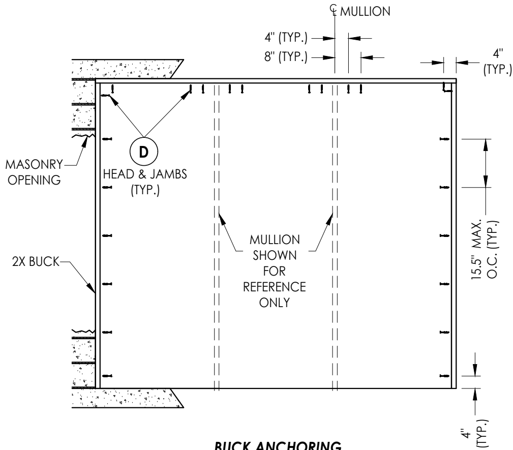
BUCK ANCHORING
