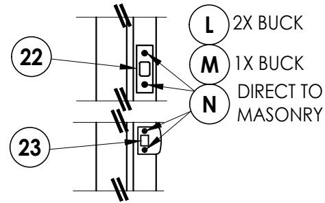
LATCH AND DEADBOLT DETAIL
