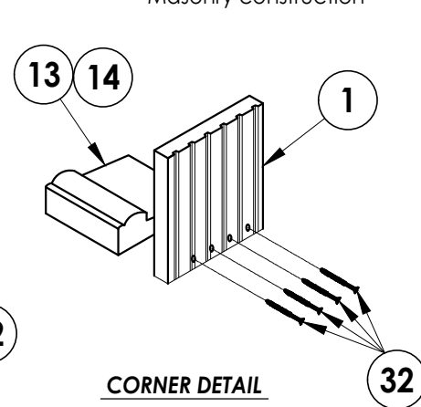
FRAME ANCHORING
