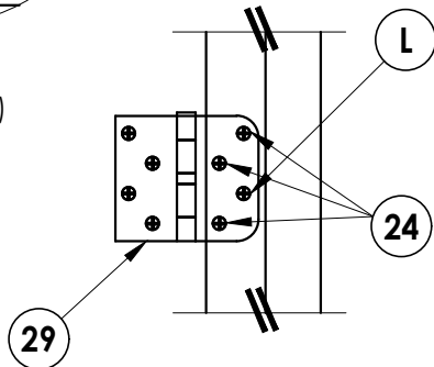
HINGE DETAIL
