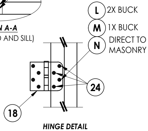
HINGE DETAIL
