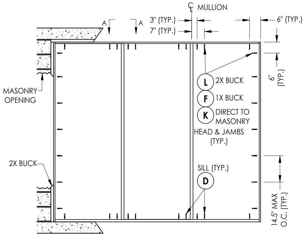
FRAME ANCHORING Masonry construction
